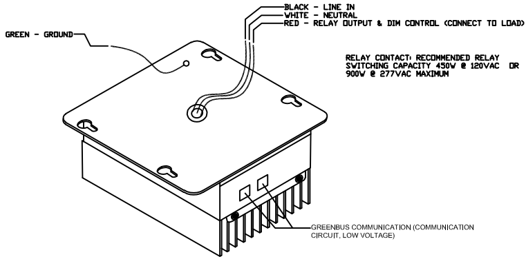
ENCELIUM PHASE CUT DIMMER MODULE (PCDM)
